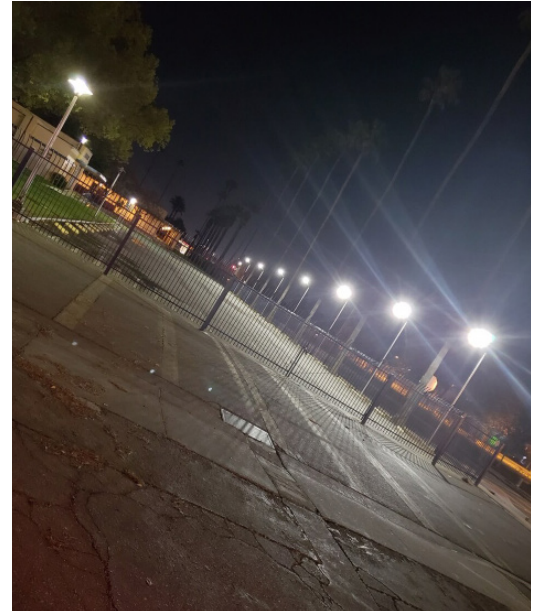
Solar Area Light - 30W, 6000 Lumens Delano High School, CA Fixture Height = 15'
